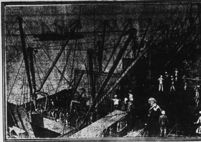
A battle ship coaling at sea is shown in this picture. The Cyclops, a navy collier, is putting a supply of coal aboard the United States armored cruiser Washington, doing the work in eight hours, and handling 2,100 tons of coal.
