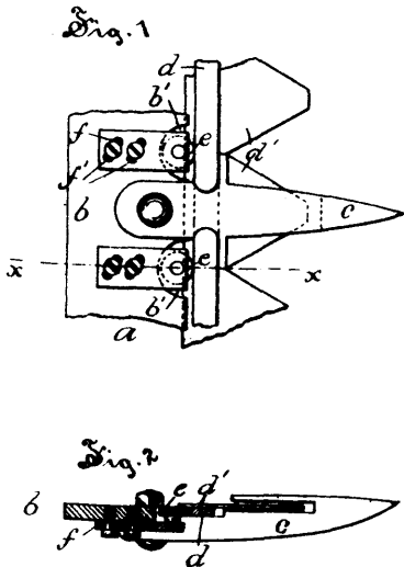
25647 Weaver's Finger Bar for Mowing Machines.
