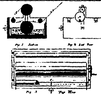
3494 Bustin's Machine for Hanging Wall-paper.
