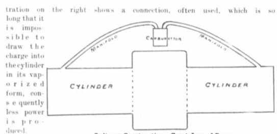
Notice in the illustration on the left the short distance from carburetor to cylinder, this means perfect combustion and greatest power; while the illustration on the right shows a connection, often used, which is so long that it is impossible to draw the charge into the cylinder in its vaporized form, consequently less power is produced.
