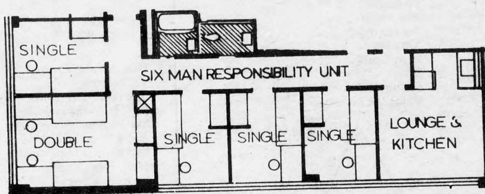
PARTIAL - FLOOR PLAN - SINGLE STUDENT RESIDENCE
