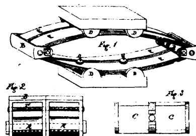
2419 Allyn's Railway Car Elliptic Spring.
