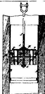
2415 Bolton &amp; Rothwell's Pump.
