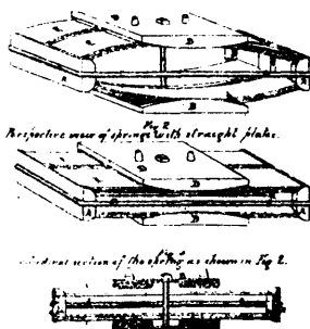
2418 Allyn's Railway Freight Car Spring.
