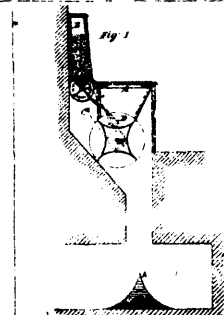
2413 Syng's Deodorizing Apparatus.
