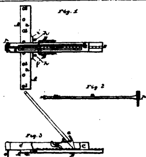
8987 Brumfield's Carpet Stretcher.
