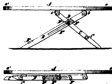
8995 Duval's Improvements in Ironing Boards.
