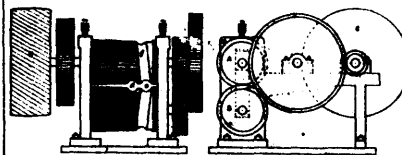
8992 Leslie's Machine for Crushing Withs.
