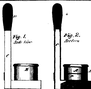
8984 Moench's Device for Ventilating Millstones.
