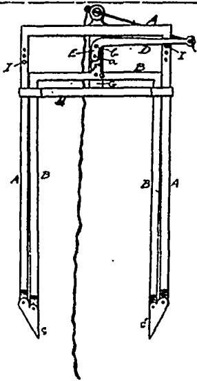
28356 Buchanan &amp; Mathieson's Hay Fork.
