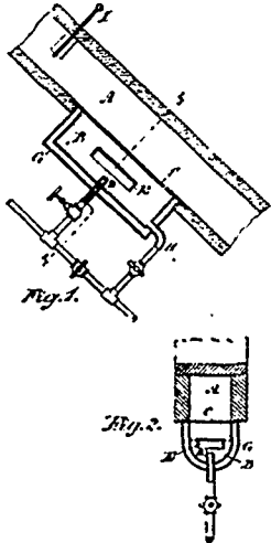
28363 Powell's Apparatus for Milling.
