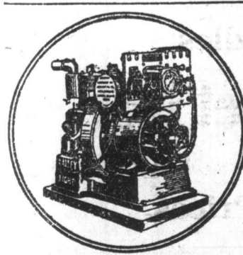
Lally-Light is a complete unit--engine and generator--with 16-cell storage battery. It supplies ample electricity for lights, motor pumps, washing machines, saws, grinders, separator, faning mill, iron, etc.
