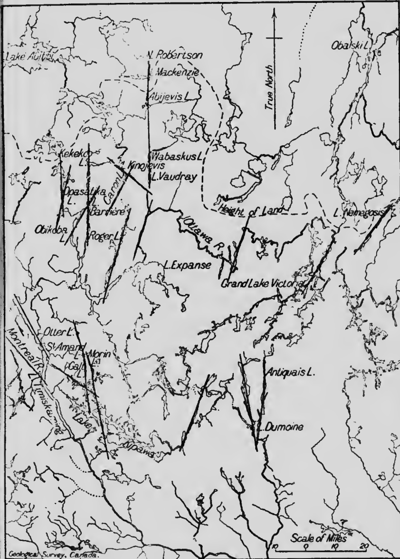
Figure 3. Linear valleys unrelated to rock structure, Timiskaming county.
