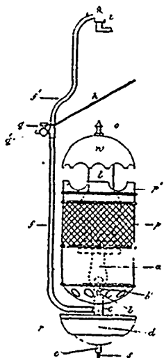
28516 Miller's Gas Heating Apparatus.
