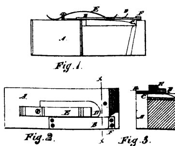
Fig. 1. Fig. 2. Fig. 3. Richmond's Machine for Shaving Feathers.
