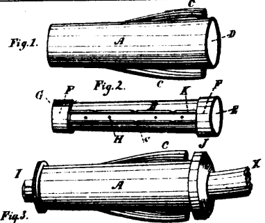
Fig. 1. Fig. 2. Fig. 3. Drew's Improvements in Axle Boxes.
