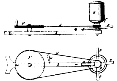
5837 Harris' Seed Sower.
