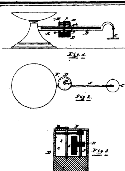
22588 Irvine's Indicating Poise for Lever Scales.
