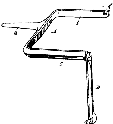
22591 Leadley's Conductor Pipe Hook.
