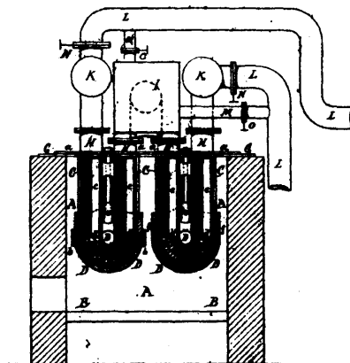
22593 Carvalho's Apparatus for Heating Air, Steam, or other like Mediums.
