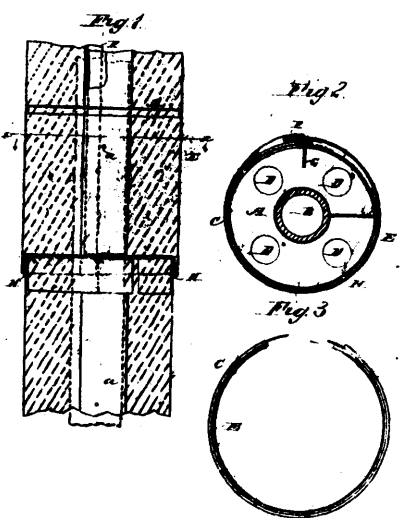
22594 Wood's Casing for Pipes.
