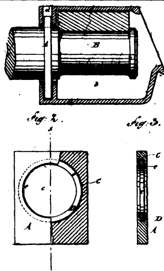
22590 Baker's Dust Guard for Railway Car Axles.
