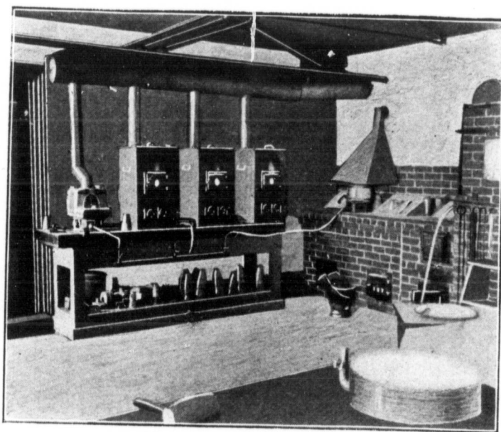
FURNACES—ASSAY LABORATORY.
