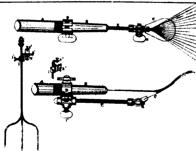
5087 Lightfoot &amp; Copping's Lawn Sprinkler.
