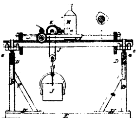
5086 Force's Device for facilitating Excavations for Sewers.
