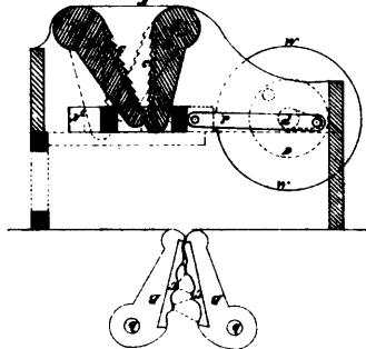
5078 Alexander's Improvements on Ore-Crushers.
