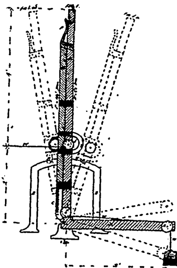
29635 Tapley's Semaphore Lever
