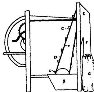
3627 Sweltzer's Fanning Mill.
