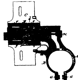
3619 Hinkley's Improvements on Saw-guides.
