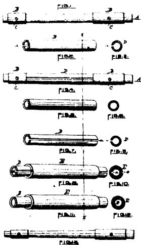
35489 Smith's Manufacture of Seamless Hollow Wire.
