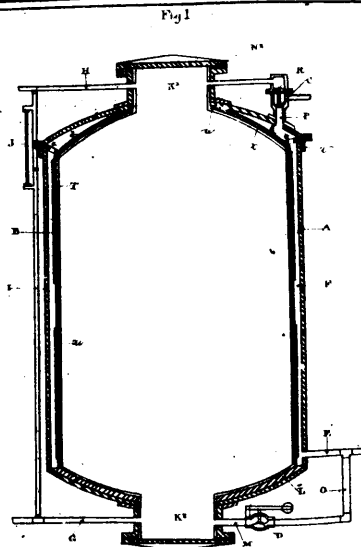
35022 Howell's Sulphite Digester for the Manufacture of Cellulose.
