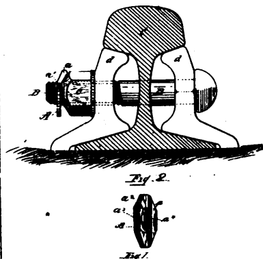
35026 Fraser's Nut Lock.
