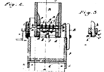
27442 Wetherby's Vegetable Cutter.
