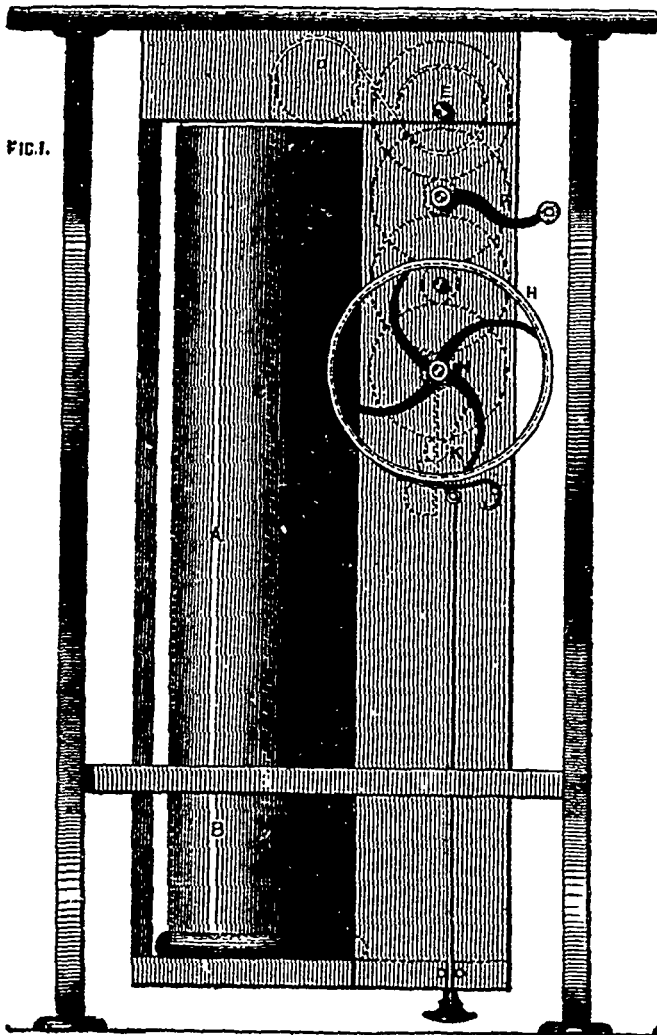
APPARATUS FOR DRIVING SEWING MACHINES. Designed by Mr. Joseph E. Holmes, Engineer, London.
