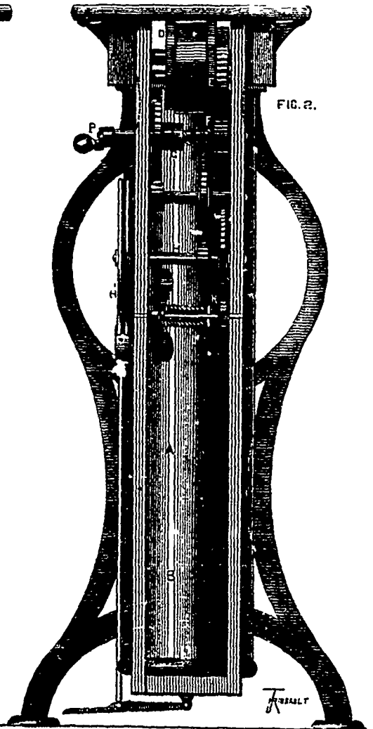
APPARATUS FOR DRIVING SEWING MACHINES. Designed by Mr. Joseph E. Holmes, Engineer, London.
