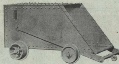
STEEL SKIPS
