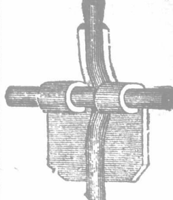
Anchor Clamp after closing
