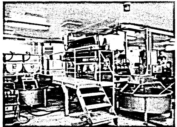
Small portion of 'surimi' processing line at Clarenville, Newfoundland plant.
