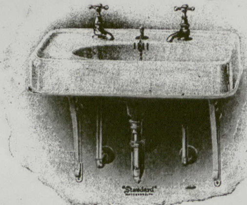
"Standard" Plate Porcelain Enamelled "Lenox" Design Lavatory with Slab, Apron, Bowl and Overflow all in one piece. Porcelain Enamelled Brackets, Nickel-plated Waste Plug, Rubber Stopper, Chain Stay and Chain, Low Pattern Compression Faucets with China Index, Supply Pipes, and "P." Trap with Waste and Vent to Wall.
