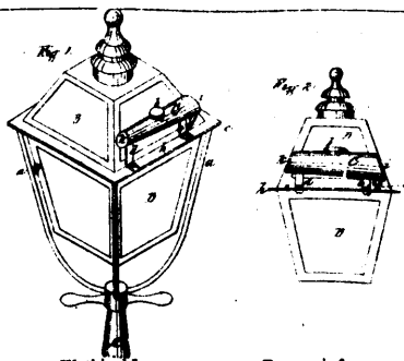
5432 Watkins' Improvements on Reservoir for Street Lanterns.
