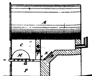
5427 Smith's Improvements on Furnaces for the Combustion of Coal.
