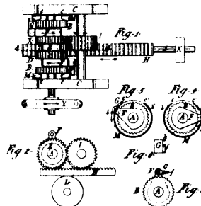
12582 Nick's Improvements in Machines for Converting Rectilinear Motion Into Rotary Motion.
