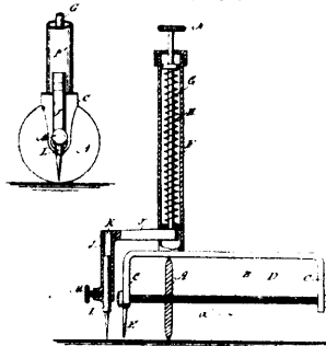
12575 D'Oopdrp's Instrument for Measuring Lines.
