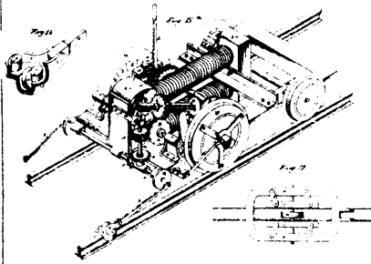
12568 Edison's Improvements on Electro-magnetic Railways.
