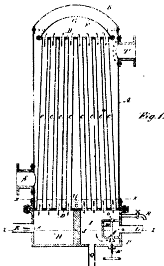
34857 Cochran & McMonagle's Feed Water Heater.
