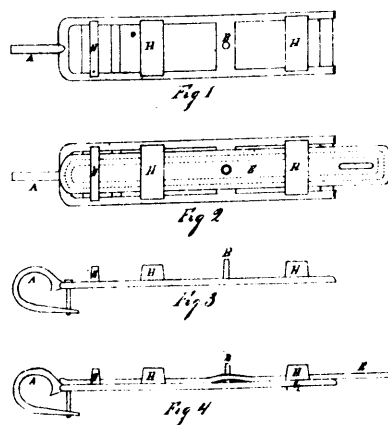
34861 Lymburner & Mathews' Connection for Trace and Hames.
