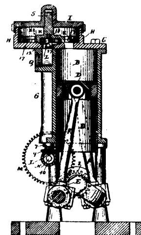
Vogel's Valve.
