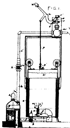
Burrow's Carbureting Apparatus.
