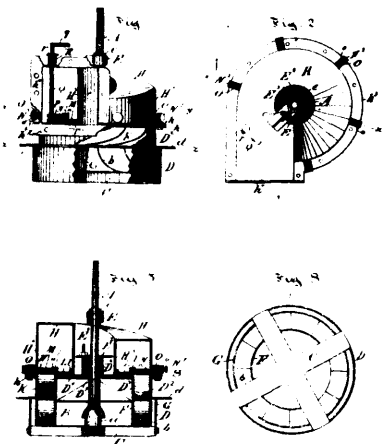
Le Bel's Turbine.
