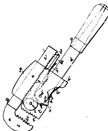
Hersey's Pipe Wrench.
