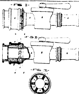
15319 Prunty's Improvements on Hose Pipe Nozzles.
