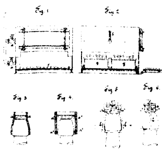
15320 Von Roden's Process and Apparatus for Preserving Milk.
