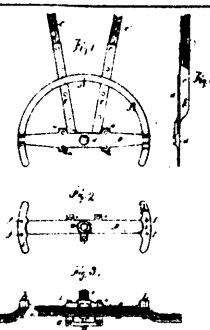
15324 Carter's Improvements on Fifth Wheels for Waggon.
