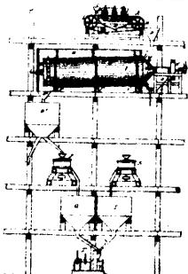
15322 Jehn's Process and Apparatus for Treating the Refuse of Starch and other Substances.
