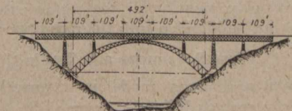
Arch over River Adda at Paderno.
