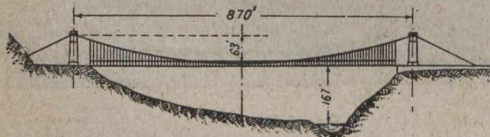
Bridge over the Sarine Valley at Fribourg, Switzerland.
