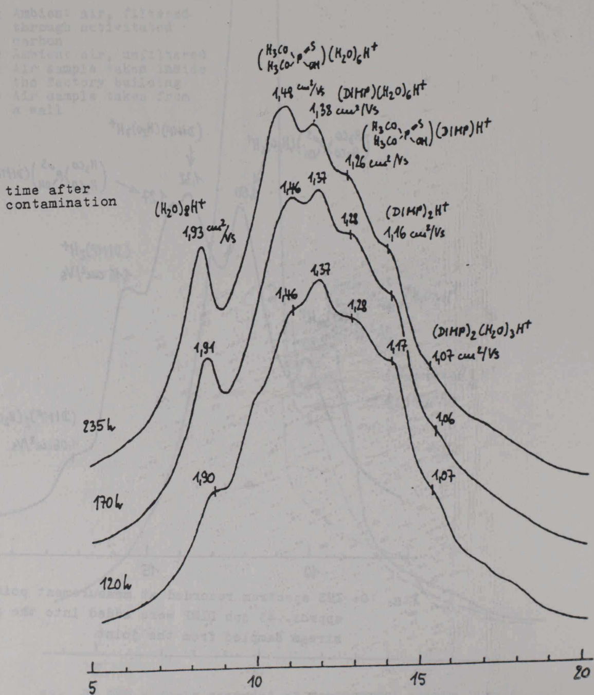
Fig. 11: IMS spectra recorded from fitting material (Kautasit), which was submerged into a parathion-methyl DIMP - mixture (1°/00) for 16 hours, time dependence
