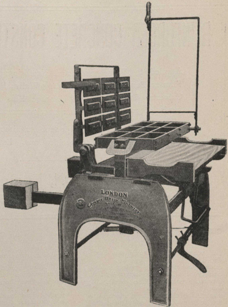
LONDON CEMENT BRICK MACHINE 5,000 Pressed Bricks per day, with one man operating
