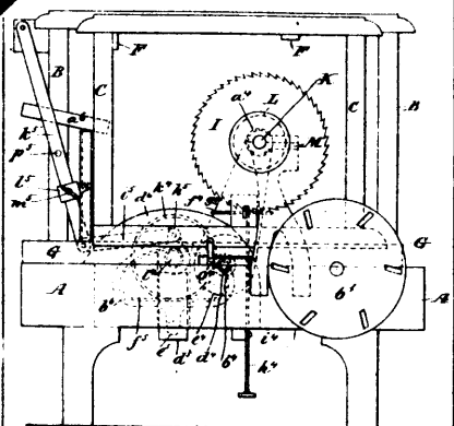
18901 Fréchette's Machine for making Shingles, &c.
