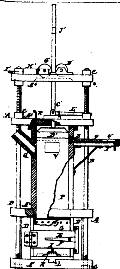
18905 Frysinger's Packer for Flour, Bran, &c.
