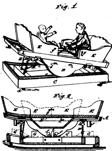
18902 Hill's Combined Cradle and Seesaw.
