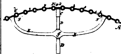
18901 Fréchette's Machine for making Shingles, &c.
