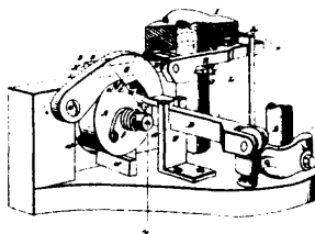
12757 Fndmore's Mechanism for Controlling the Operation of Harvester Reakes, &amp;c.
