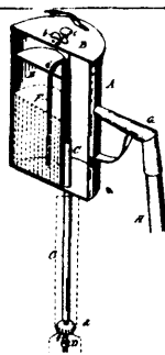
12780 Newth's Improvements in Lamp Lighters.
