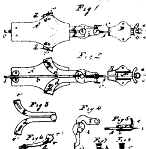
12754 Barney's Improvements in Skate Fasteners.
