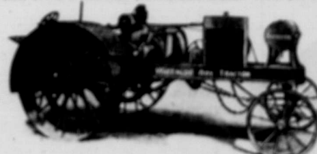
Weight only 4800 lbs. Brake Test 24 H.P.; Draw Bar 12 H.P. Ignition High Tension Dual Magnets. With Automatic Spark Advance.
