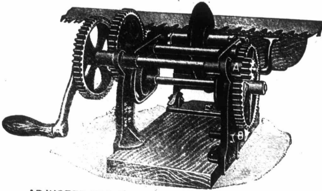
ADJUSTED FOR SAWS AND GROOVED CHISELS. $7.50 COMPLETE, INCLUDING SICKLE TOOL, SAW GUARD, WHEELS AND ATTACHMENTS.
