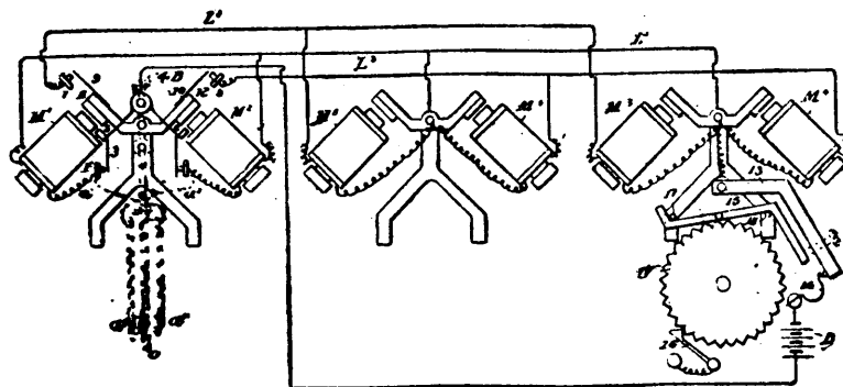
FIG. 5.—DIAGRAM OF CIRCUITS.
