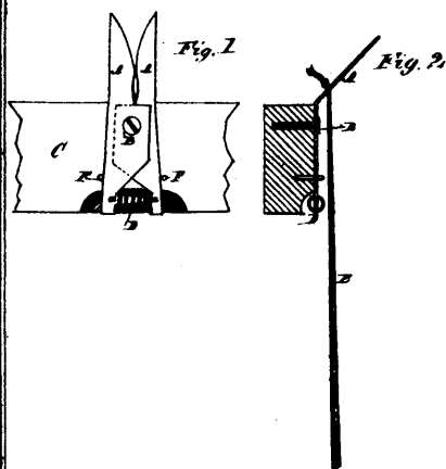
16137 Peters &amp; Swartsenburg's Improvements in Whip-Holders.
