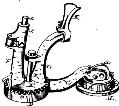
16140 Robert's Improvements in Shoemakers' Jacks.
