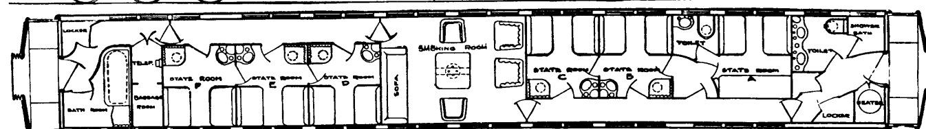
SLEEPING CAR CANADA
