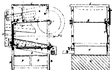
15461 Costin's Improvements on Fanning Mills.
