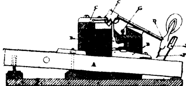
15468 Dettmann's Improvements on Plate-Forces.
