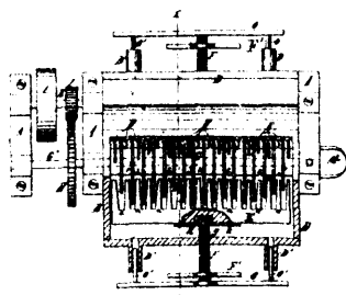
15467 Baré's Improvements on Machines for Shredding Sugar Cane.
