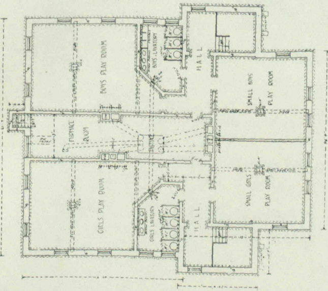
BASEMENT PLAN
