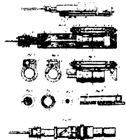
11780 Richmann & Arnold's Improvements in Rock Drilling Apparatus.
