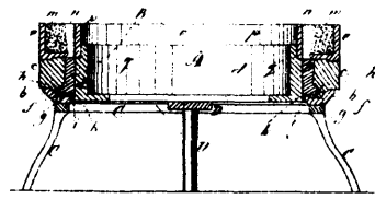
11769 Washburn's Improvements on Moulds and Processes for Casting Car Wheels.
