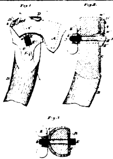
11765 Pressey's Improvements on Seythe Fastenings.
