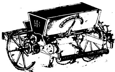
10847 Bogle's Improvements on Grain Sowers.
