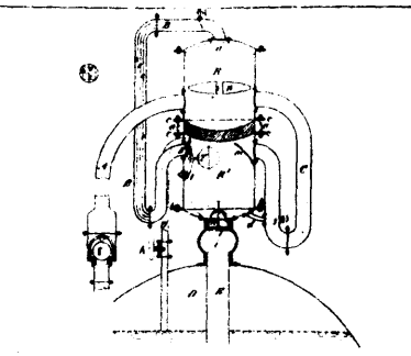
5257 Yaga's Improvements on Feeding Apparatus of Steam Boilers.
