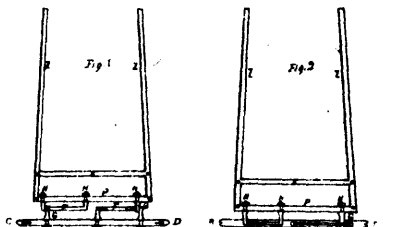
5262 Wood's shaft-coupling for Cutters.
