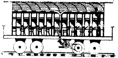
5252 Hargreaves' Railway Car Ventilator.
