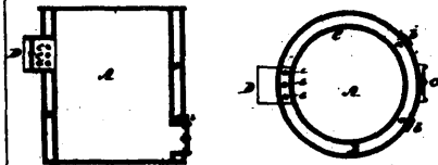
3896 Lingenselter's Portable Furnace.
