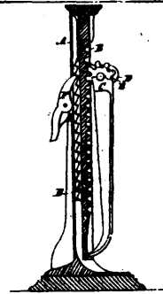
3891 Scott's Carriage Lifting Jack.
