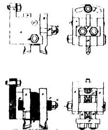
3243 Carr & Turbull's Improvements in Tool Boxes and Cutters for Iron Planers.
