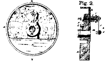
14973 Rice's Improvements on Valve Gear for Engines.
