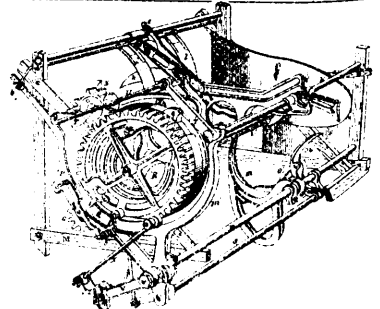
14970 Whiteley & Bailey's Improvements on Harvesters and Binders.
