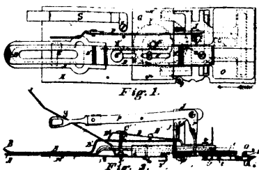
14978 Baird's Improvements on Button Hole Attachments for Sewing Machines.
