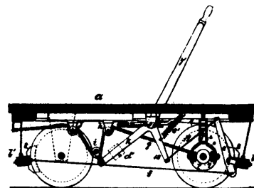
7956 Gu &amp; Field's Improvements on Railway Brakes.
