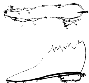
7950 Horsford's Improvements in Ice Creepers.
