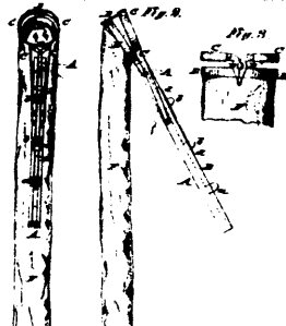
7955 Sager &amp; Gerlach's Improvements on Fruit Pickers.
