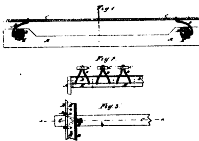
7952 Edmans' Spring-Bed Bottom.
