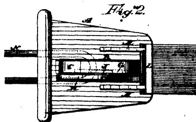
Johnson and Walkey's Car-Coupling.
