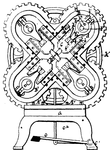
Richardson's Radial Forging Machine.
