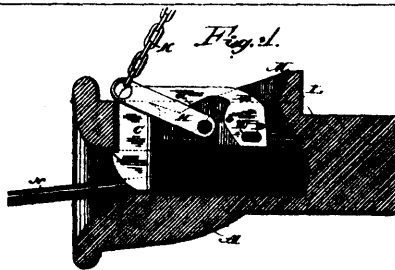
Richardson's Radial Forging Machine.
