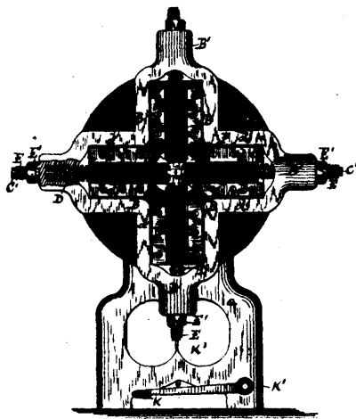
Richardson's Radial Forging Machine.
