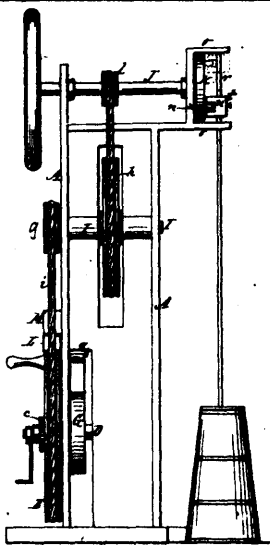
Furlong's Motive Power.
