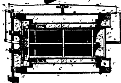
Walter's Middlings Purifier
